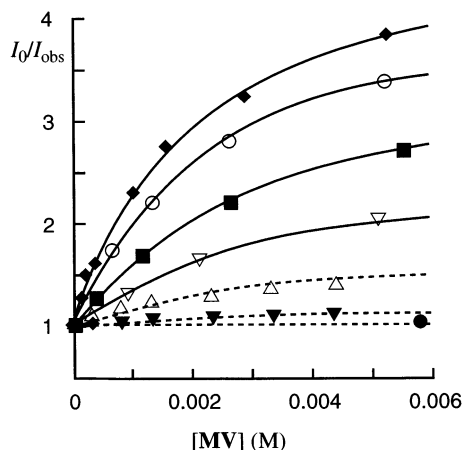
Fig. 2. Stern–Volmer plots for the fluorescence quenching of zinc porphyrin in the myoglobin upon addition of MV at 10 mM phosphate buffer at 25°C. The solid lines correspond to the data obtained in rMb(1·Zn): pH 5.8 ( \nabla ); pH 6.1 ( \blacksquare ); pH 6.4 ( \circ ); pH 7.1 ( \blacklozenge ). [rMb(1·Zn)] = 10^{-6} M. The dashed lines correspond to the data obtained in rMb(2·Zn): pH 7.0 ( \bullet ); rMb(3·Zn): pH 7.0 ( \blacktriangledown ); rMb(4·Zn): pH 7.0 ( \triangle ). [rMb(2·Zn)] = [rMb(3·Zn)] = [rMb(4·Zn)] = 10^{-6} M. The changes of fluorescence emission were monitored at 584 nm ( \lambda_{\text{ex}} = 543 nm).
